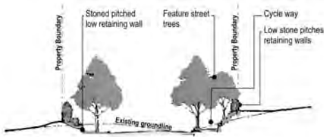
Sketch Section - Cumbalum Way
